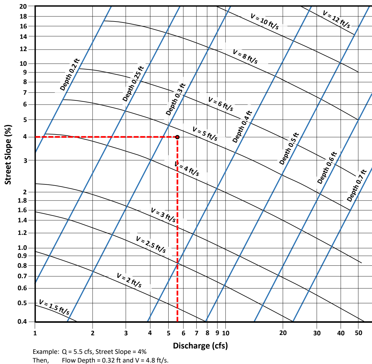
Figure 3-3. Street Gutter Flow Velocity (San Diego County, 2003)
