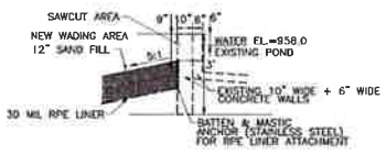
D SAWCUT DETAIL
