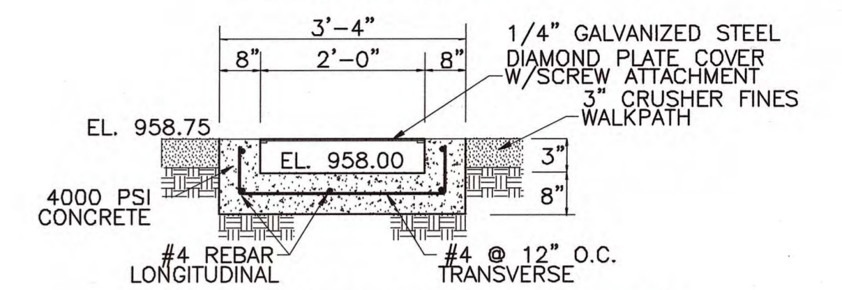
(B) NEW OVERFLOW SPILLWAY
